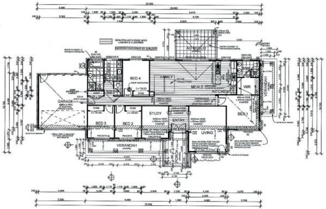
GROUND FLOOR PLAN SCALE: 1:100 @A2
