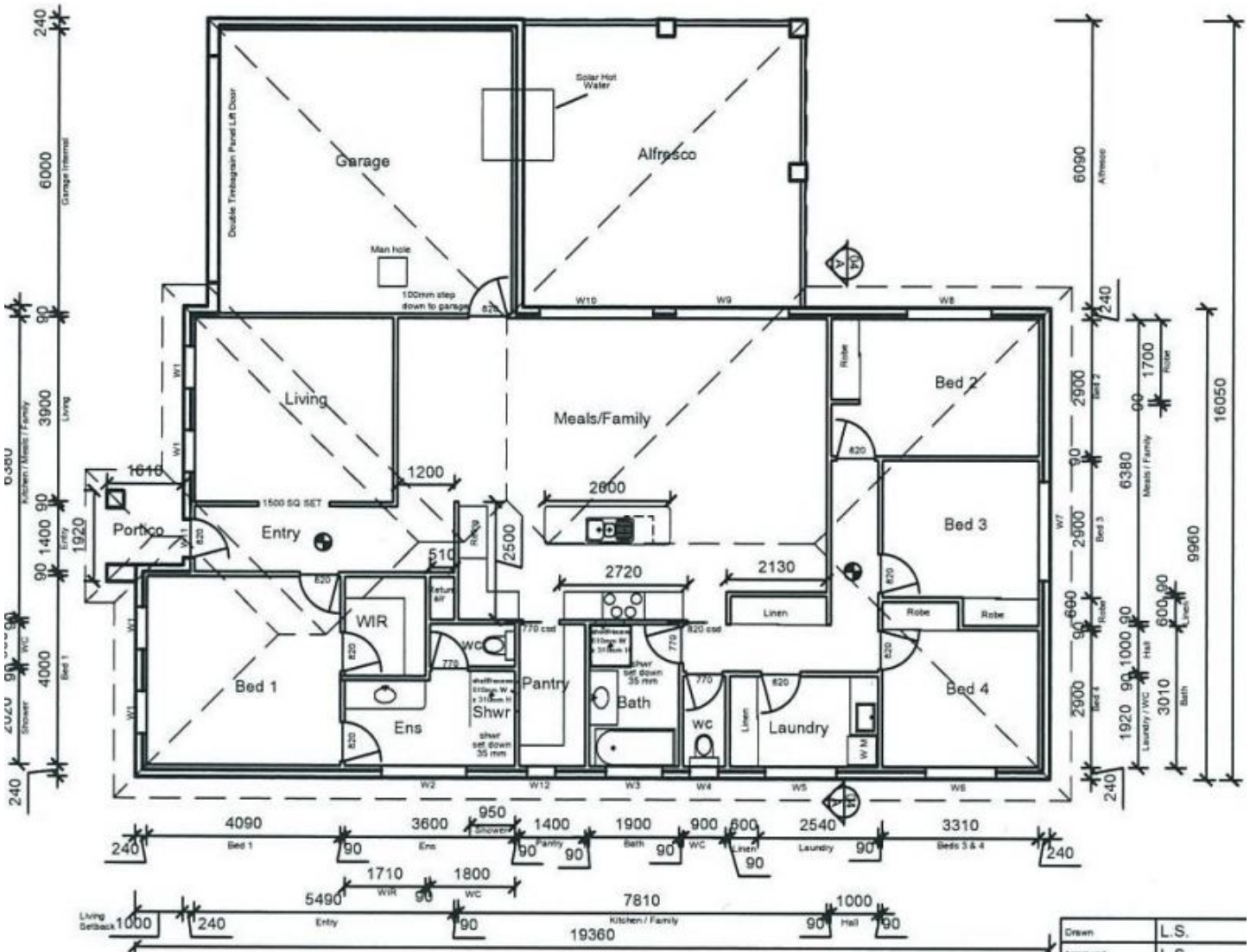
FLOOR PLAN 1/100
